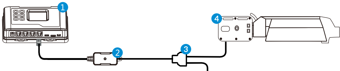
1. Controller 2. Lighting Control Adapter P 3. Splitter 4. P Ballast
